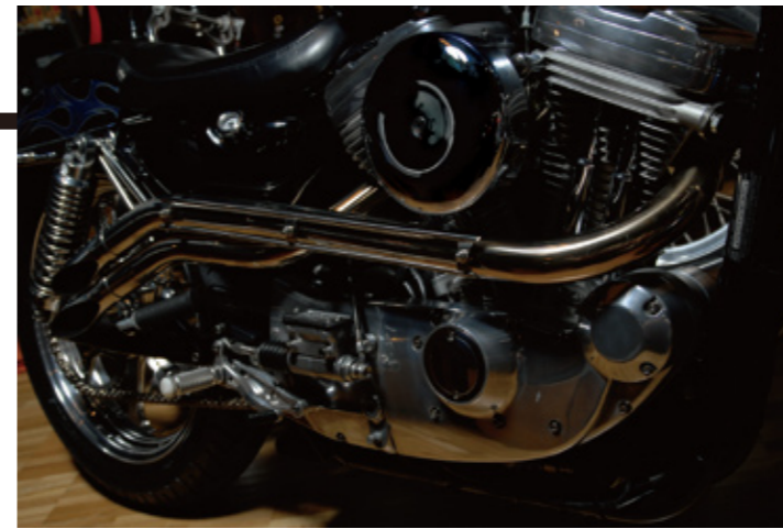
◀ Example of use of bent pipes. Type : SPORTSTER The bent pipes used in this example Front:φ45×160°/20°/40°/60° Rear:φ45×60°/40°/60°
